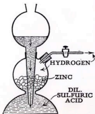
Figure 11. A Kipp's generator for generating H_2 , H_2S and many other gases. From First Principles of Chemistry , by Raymond Brownlee, William Hancock, Robert Fuller, Michael Sohon and Jesse Whitsit, Allyn and Bacon, 1931.
